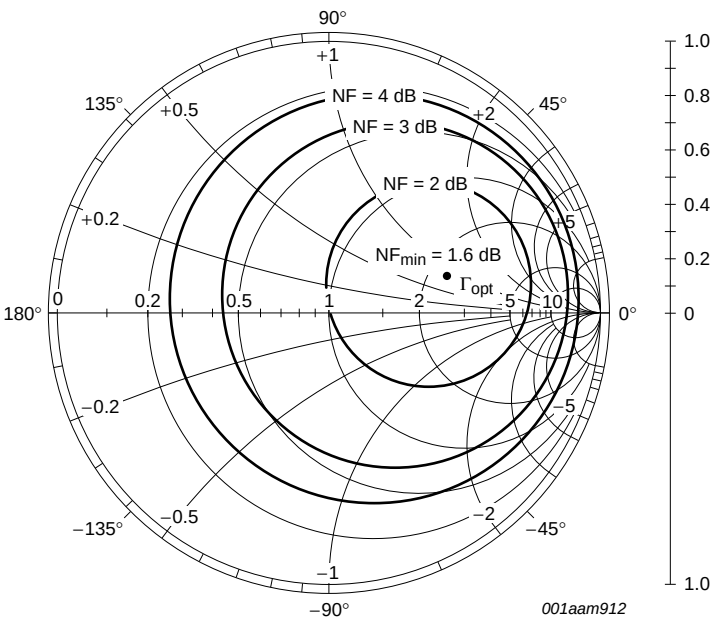
Fig 11. Common emitter noise figure circles; typical values
